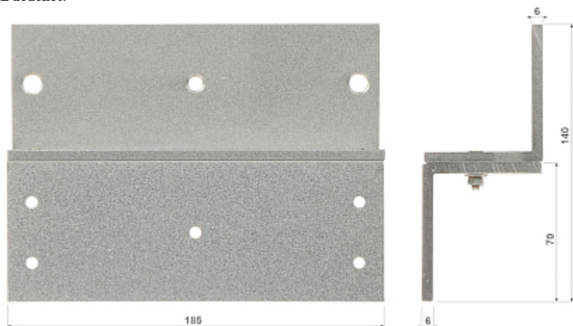
Z-bracket:
