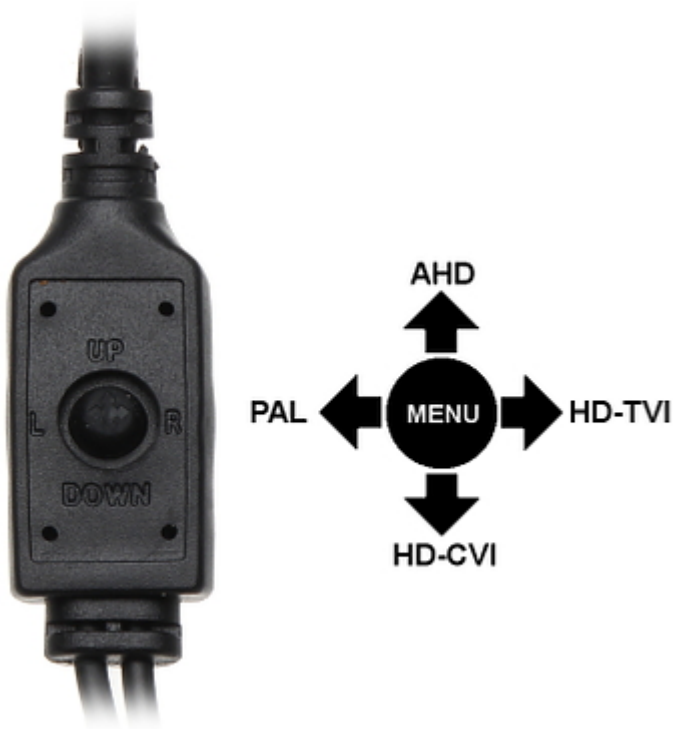
Bracket view:
