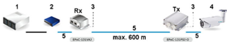
Transmission schematic diagram:
