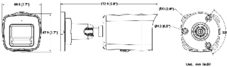
Camera mounting dimensions:
