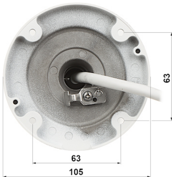
Camera dimensions:
