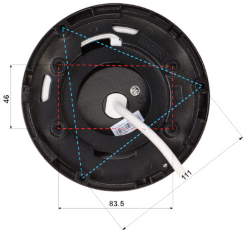
Camera dimensions:
