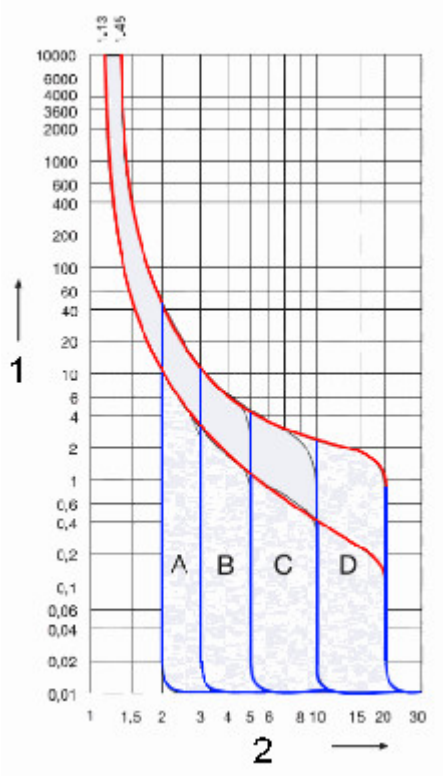
Tripping curves:
