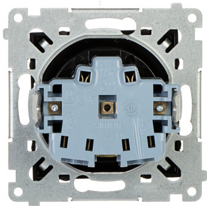
Connectors view:
