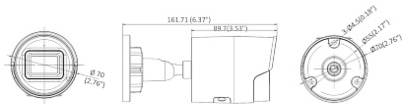
Camera mounting side view:
