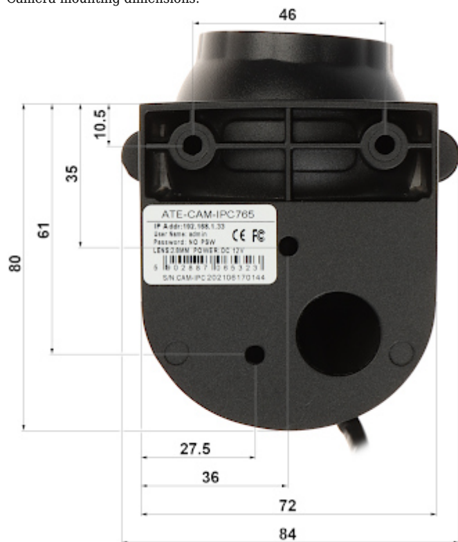
M12 connector:
