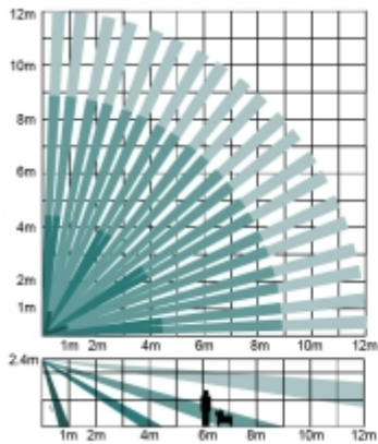
Mounting side view:
