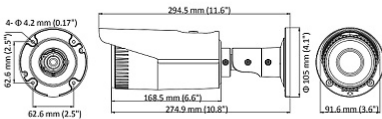
Camera dimensions:
