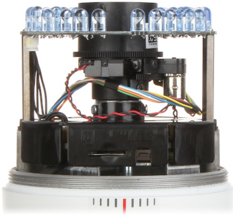
Side view:
