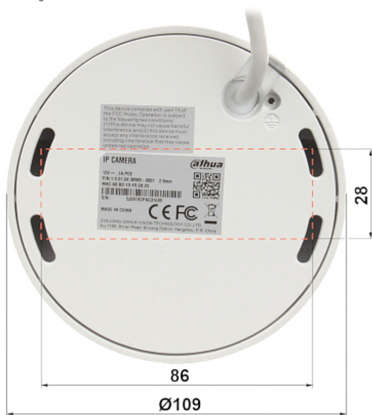
Camera dimensions:
