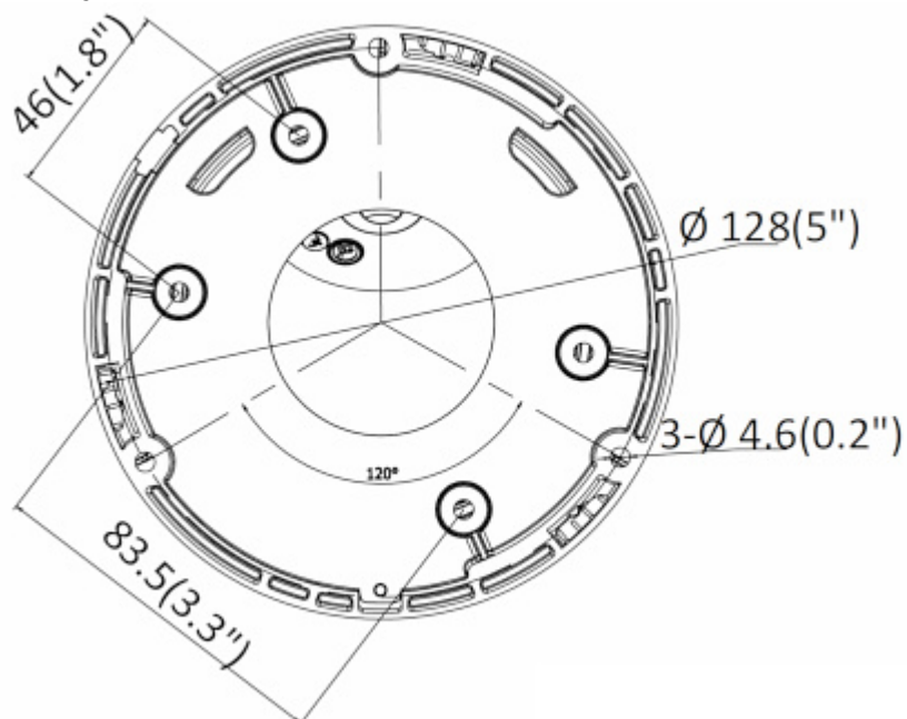
Camera dimensions:
