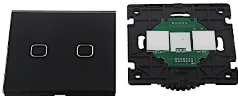
Rear view:
