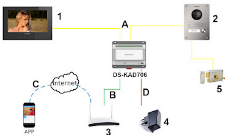
Connection schematic diagram:
