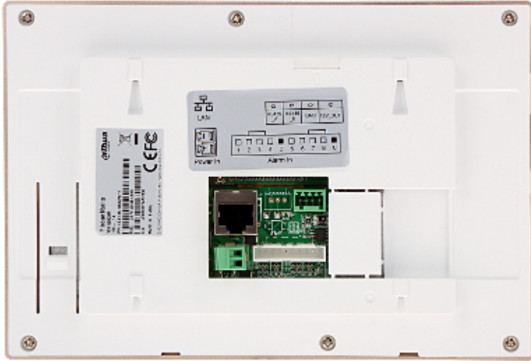
Connectors view:
