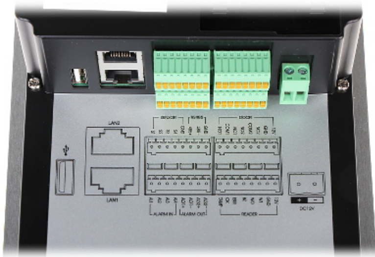
Connectors view:
