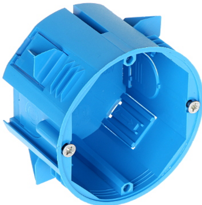
Electrical installation box to insulation of building (Styrofoam). The box is made from non-halogen, self-extinguishing plastic.
