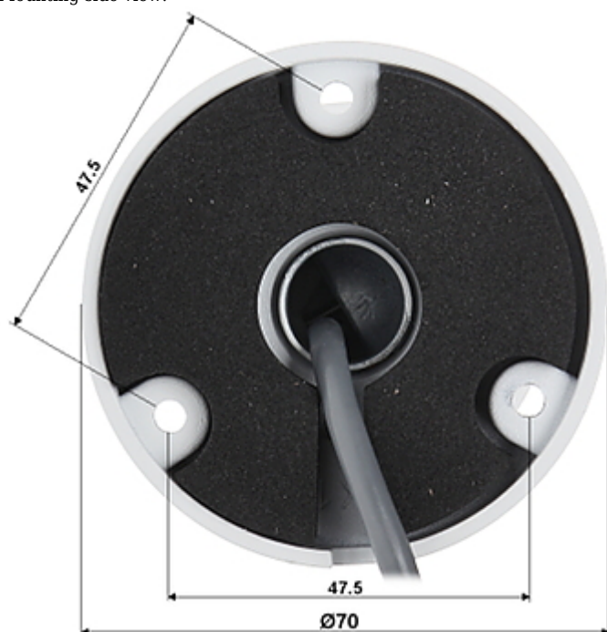
Camera dimensions:
