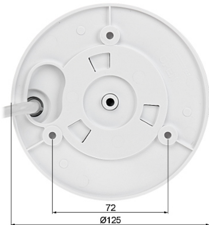
Dimensions:
