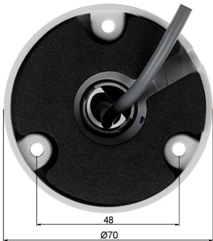
Camera dimensions:
