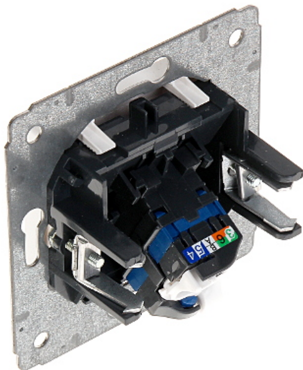
Rear view:
