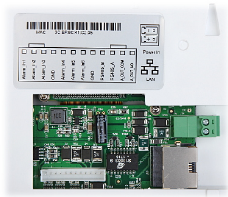
Connectors view:
