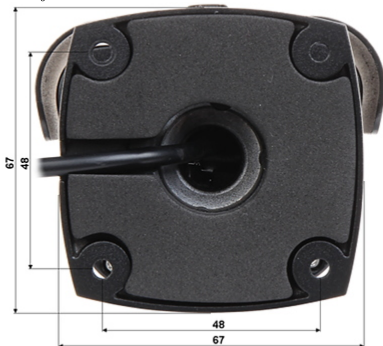
Mounting dimensions:
