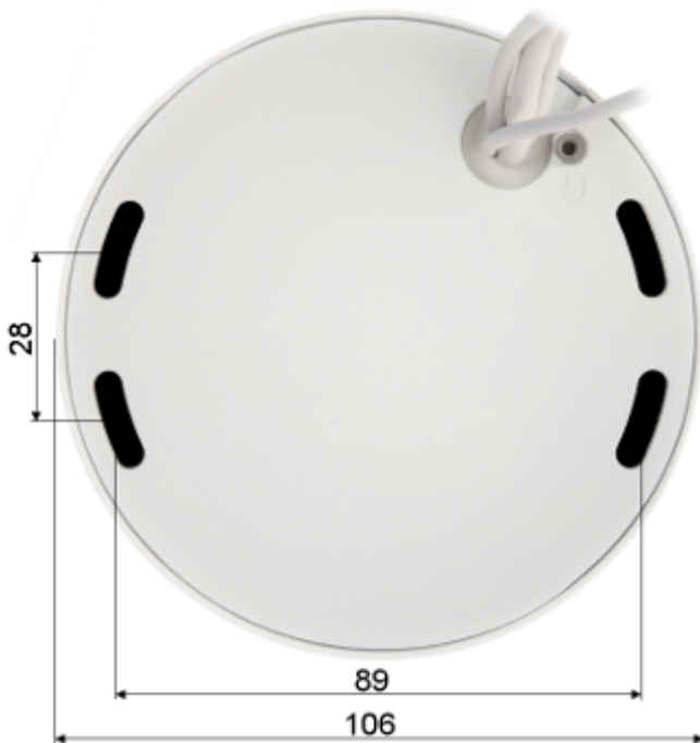
Connectors description:
