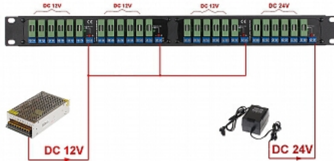
Schematic diagram of distributor application with two different voltages option:
