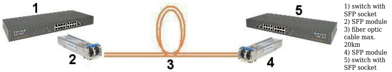
Connection diagram:
