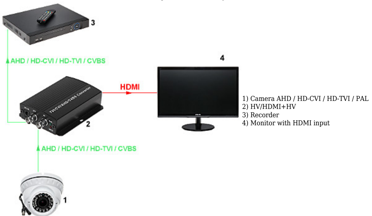
Schematic diagram of converter operation:
