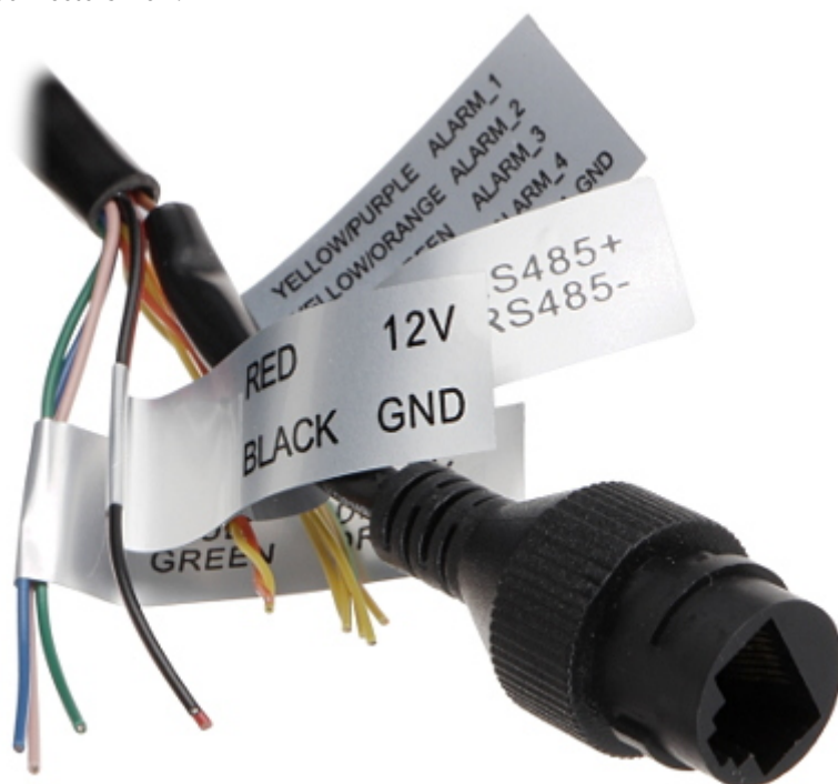
Connectors view:
