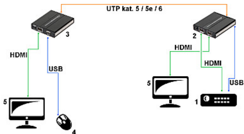
Connection schematic diagram:
