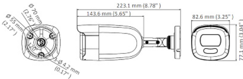
Camera dimensions:
