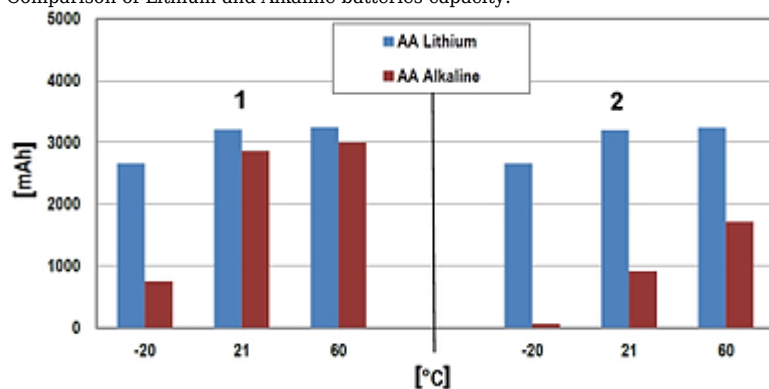
Comparison of Lithium and Alkaline batteries capacity:
