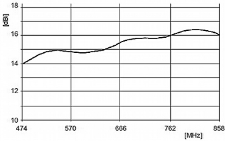
Gain versus frequency response:
