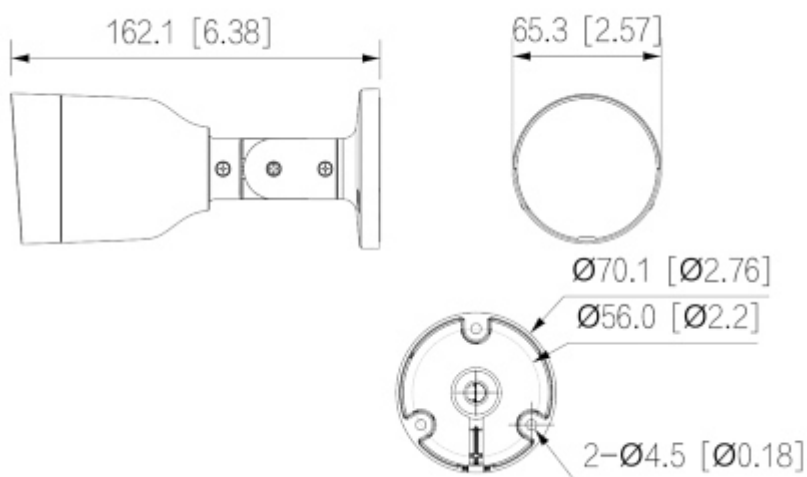
Camera dimensions:
